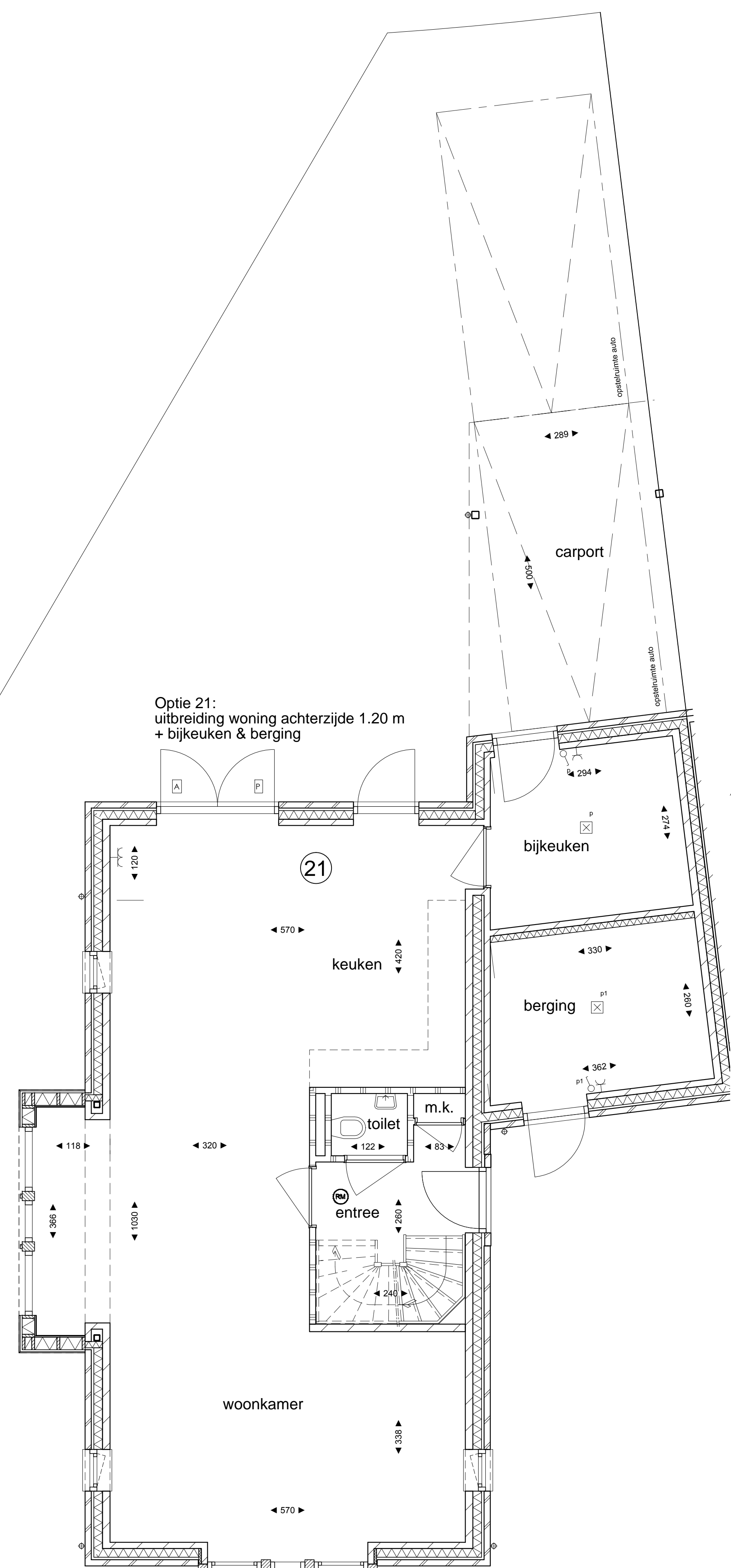
Begane-grond, kavel 5
